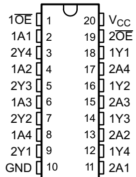
SN54AHC244 . . . J OR W PACKAGE SN74AHC244 . . . DB, DGV, DW, N, NS, OR PW PACKAGE (TOP VIEW)
