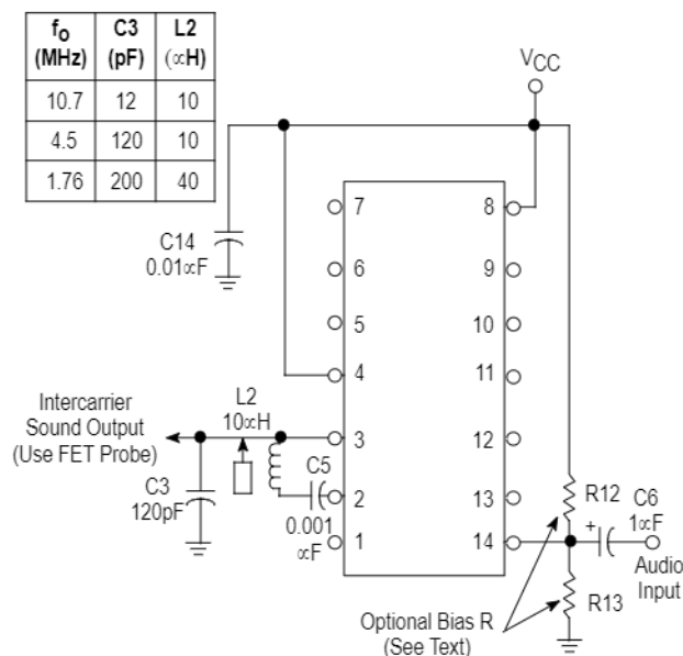
Figure 11. FM Test Circuit
