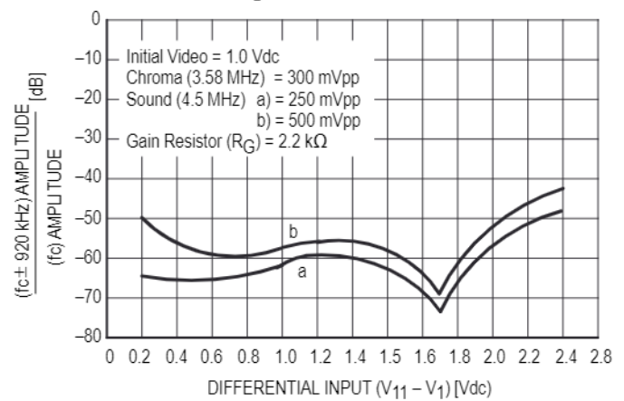
Figure 10. 920 kHz Beat
