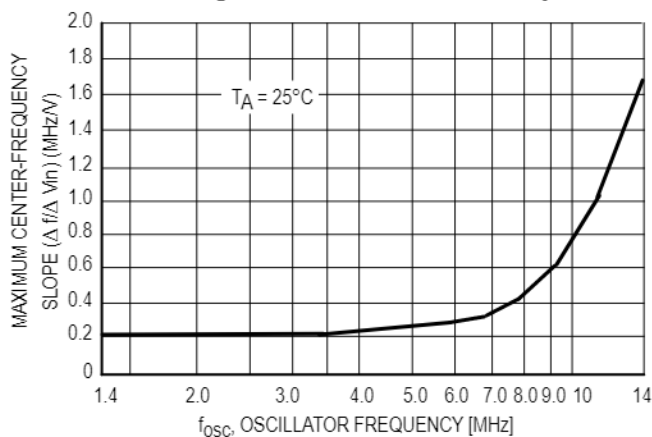
Figure 12. Modulator Sensitivity
