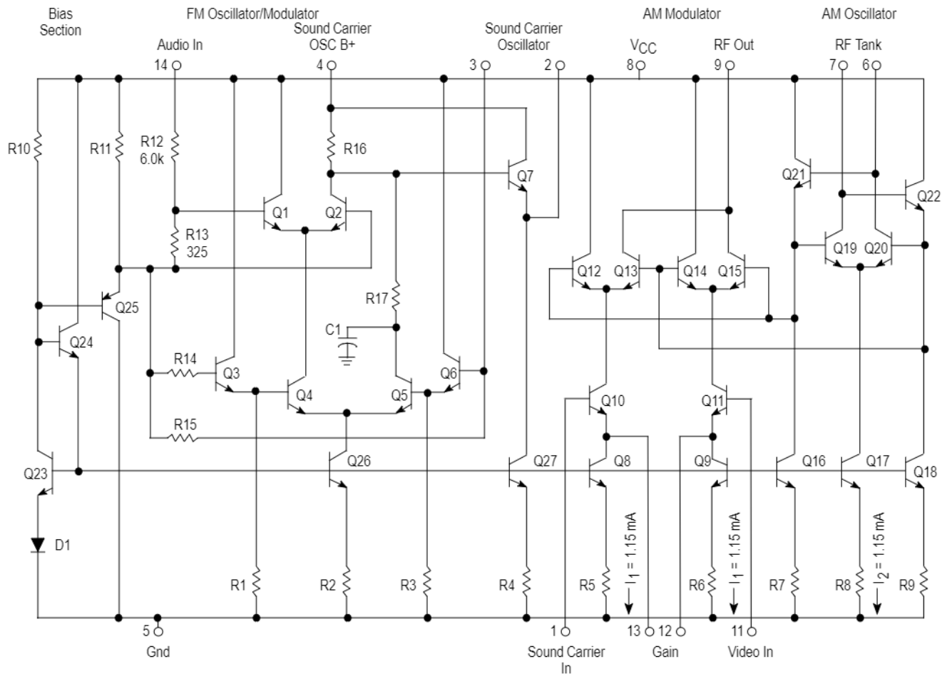
Figure 2. TV Modulator
