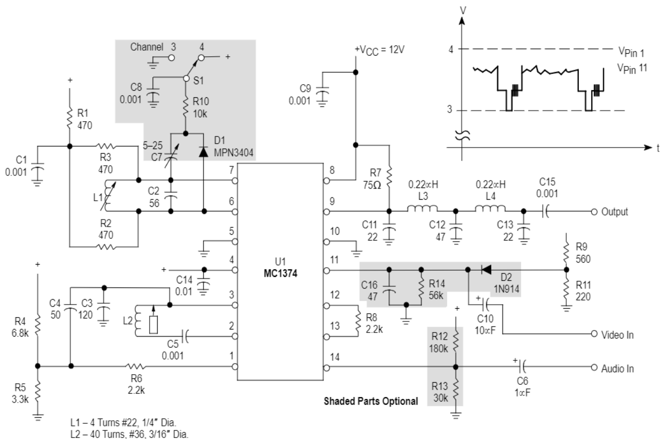
Figure 1. Simplified Application
