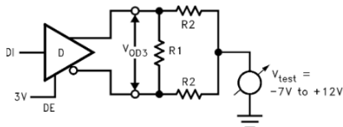
FIGURE 2. V_{OD3}
