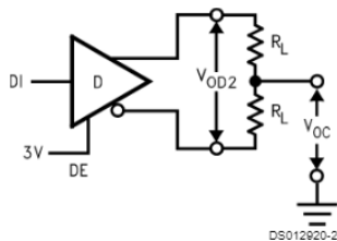
FIGURE 1. V_{OD}
