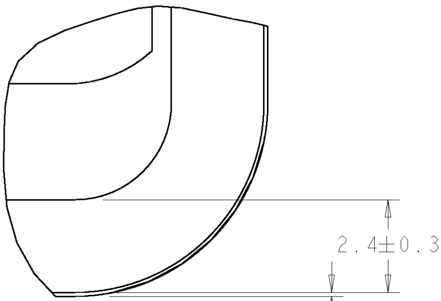
DETAIL Z SCALE 10:1
