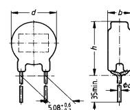
Outline drawing
